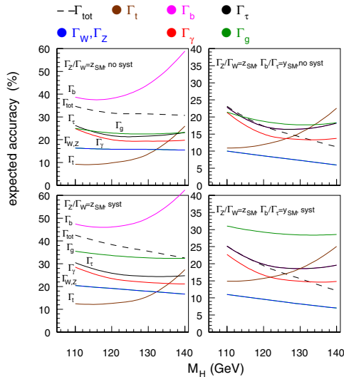
Fig. 1. Relative accuracy (%) on the individual rates \Gamma_i expected at the LHC (from [28]). See the text for a detailed description of the panels
